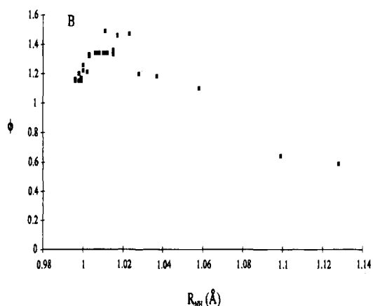
Figure 5. Fractionation factors ( \phi ) vs (A) hydrogen-bonded N-O and (B) N-H distances. The apparent maxima can be understood by the initial increase of \phi upon weak hydrogen bonding and subsequent decrease as the hydrogen bonding becomes stronger.
